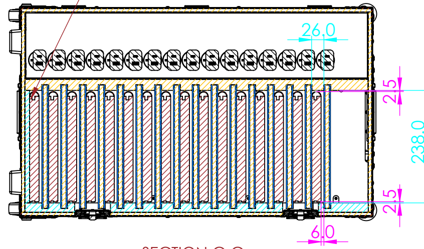
SECTION C-C
