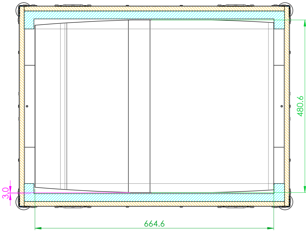
SECTION B-B
