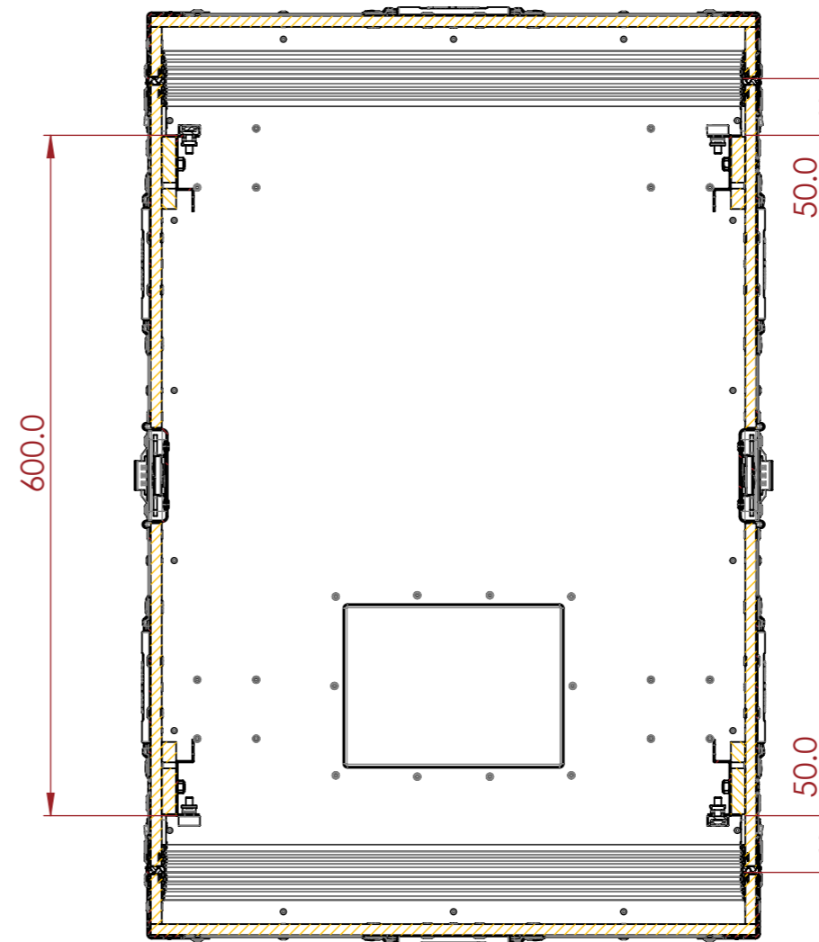
SECTION B-B
